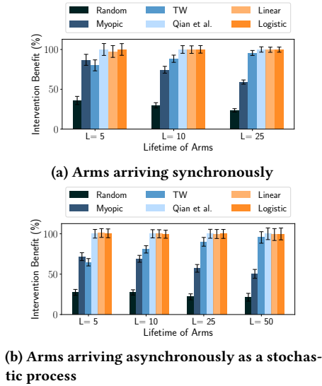
Figure 3: (a) Performance of Threshold Whittle algorithm degrades when the lifetime of arms gets shorter, even when all arms start synchronously (b) The performance dwindles further if arms arrive asynchronously.
